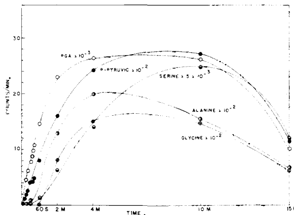
Fig. 4.—CO 2 fixation in the two- and three-carbon compounds during photosynthesis by Scenedesmus at 15° (10 cu. mm. cells).
