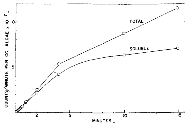
Fig. 2.— \text{CO}_2 fixation by Scenedesmus during photosynthesis at 15°.
