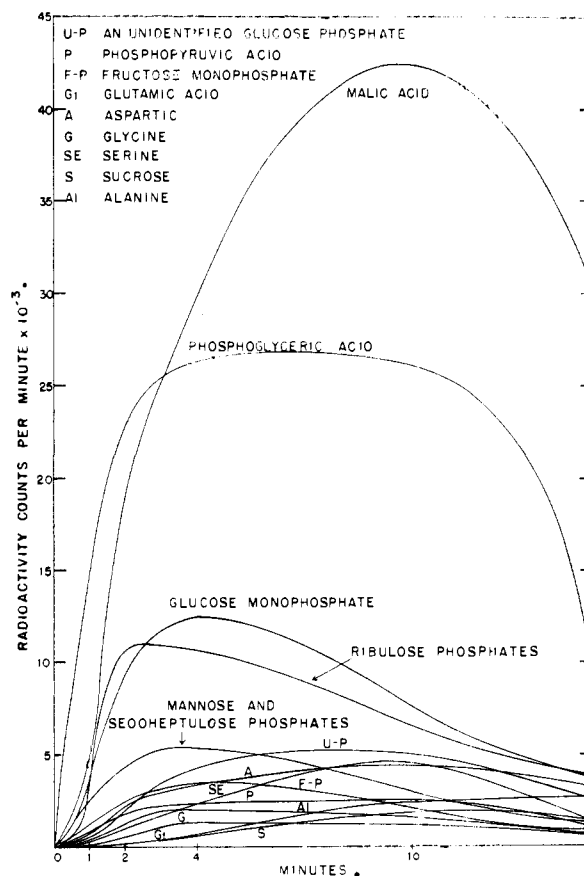
Fig. 7.— CO_2 fixation in the major soluble compounds in the same scale during photosynthesis by Scenedesmus at 15^\circ (10 cu. mm. cells).
