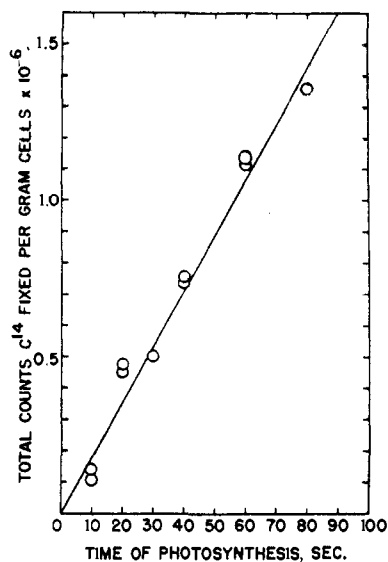
Fig. 1.— \text{CO}_2 fixation by Scenedesmus during photosynthesis at 2°. The curve represents the total fixed and there was no appreciable insoluble reaction product at the time interval shown.
