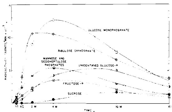
Fig. 5.—CO 2 fixation in the sugar phosphates and sucrose during photosynthesis by Scenedesmus at 15° (10 cu. mm. cells).
