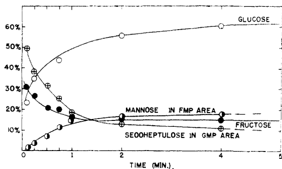
Fig. 8.—Percentage distribution of fixed carbon among the sugars, glucose, fructose, mannose and sedoheptulose during photosynthesis by Scenedesmus at 15°. The distribution of total count in the heptose area between mannose and sedoheptulose shown above was made from the ratio of these two substances as determined in Fig. 3.
