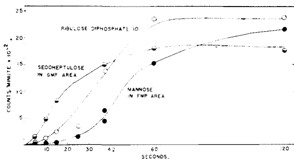
Fig. 3.—Radioactivity incorporated in the heptose phosphate areas and the ribulose diphosphate area during photosynthesis by Scenedesmus at 20°. (10 cu. mm. cells). The sedoheptulose is contaminated with some mannose and the mannose is contaminated with some sedoheptulose as they are given here.
