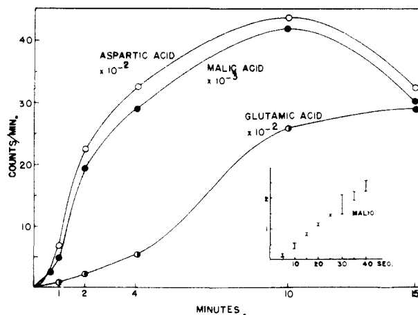
Fig. 6.—CO 2 fixation in the four-carbon acids and glutamic acid during photosynthesis by Scenedesmus at 15° (10 cu. mm. cells).
